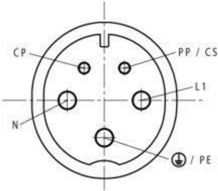
Front view of pins of vehicle inlet
