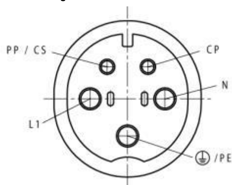
Front view of contact tubes of socket- outlet
