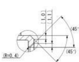
DETAIL L
