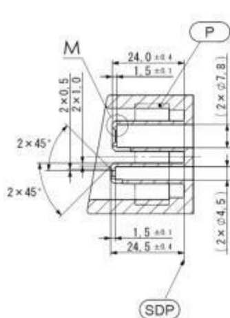
SEC.J-J
